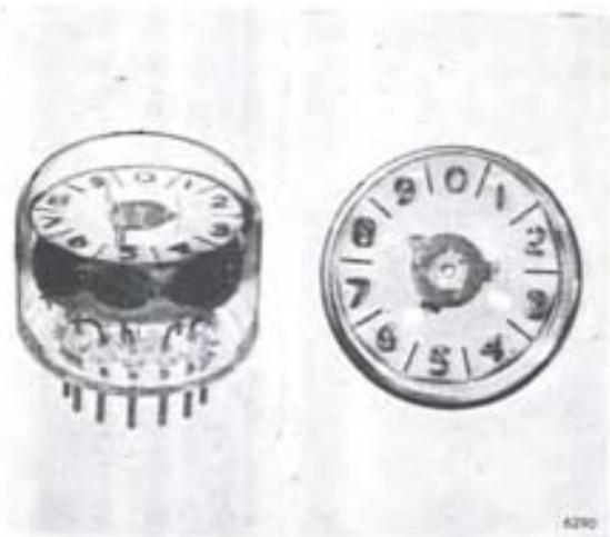
Fig. 4. Photographs of the Type Z 550 M indicator tube.
